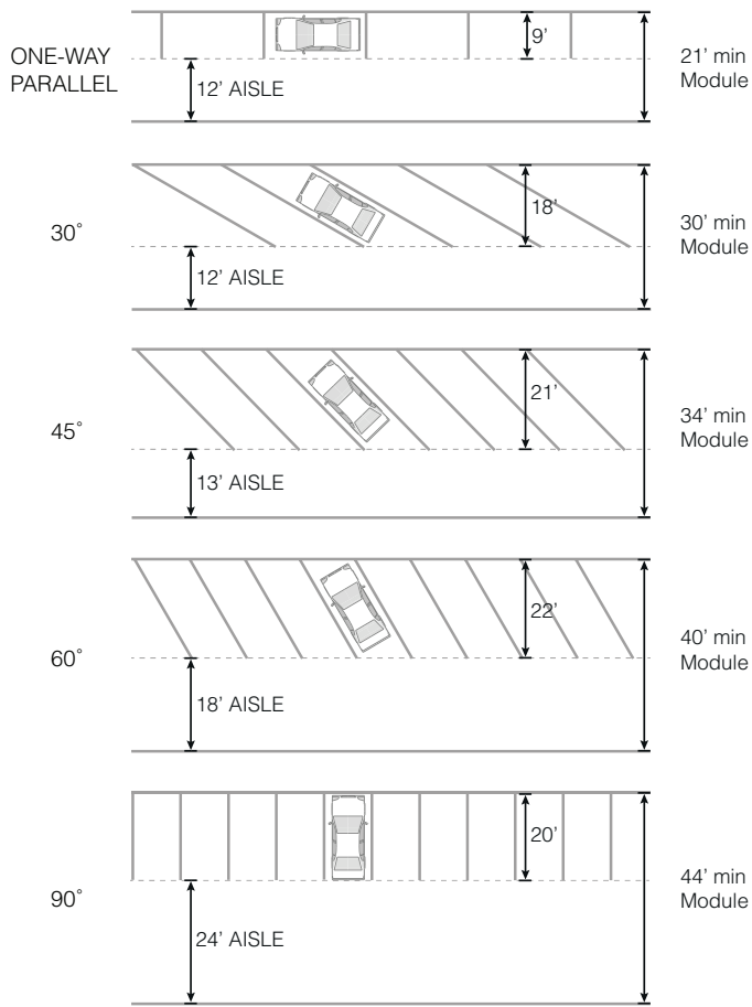
One Row of Parking
