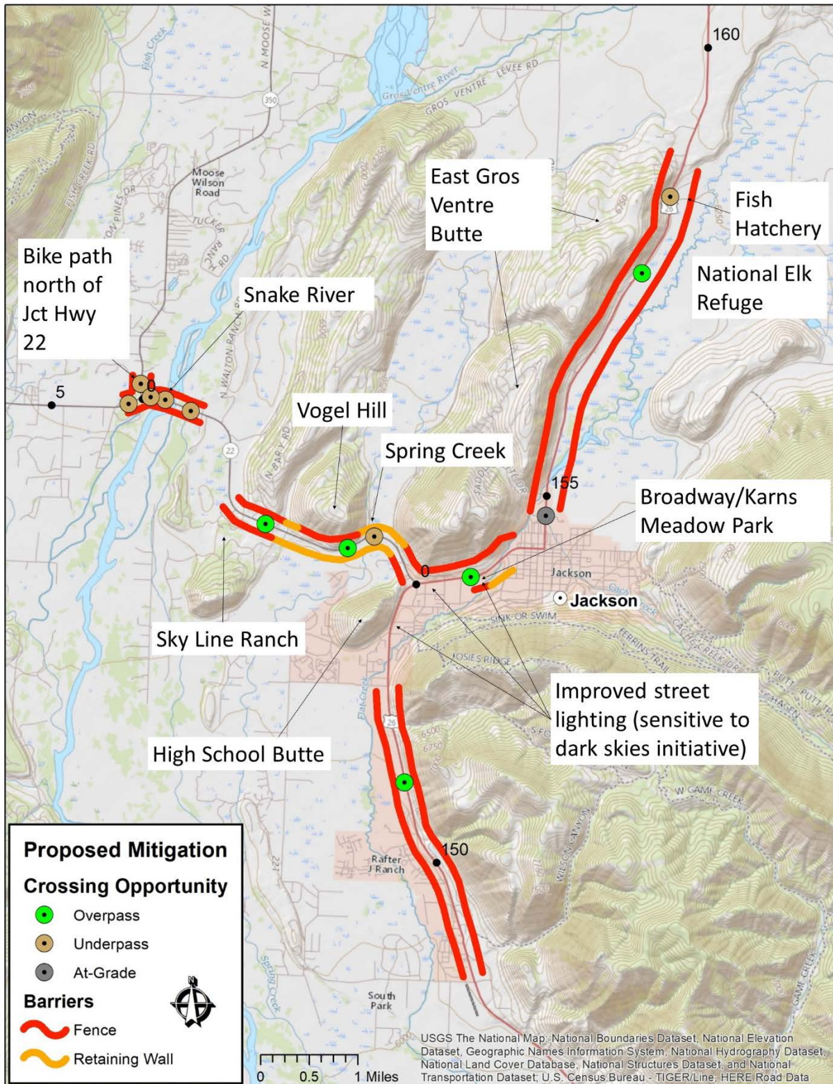
Figure 31. Suggestions for potential future mitigation measures (zoomed in around Jackson). Note that the wildlife fences in combination for wildlife crossing structures is the preferred option over at-grade crossing opportunities
